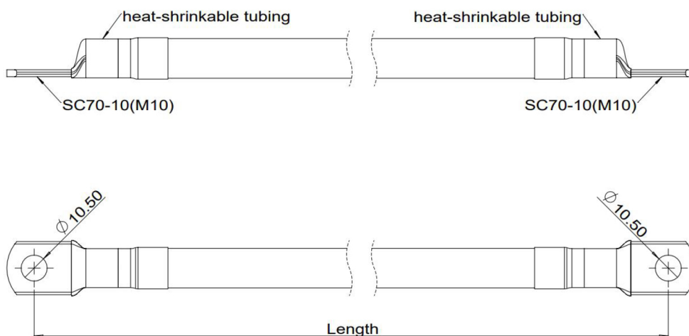
00AWG Power Cable
