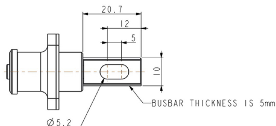
Busbar Termination
