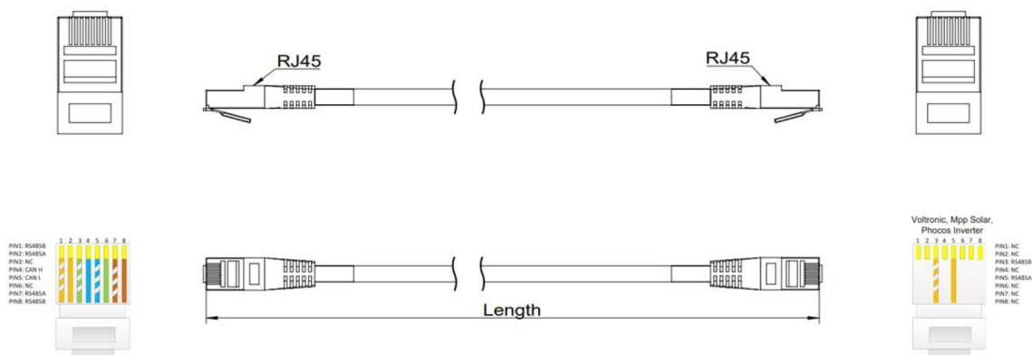
Voltronic Off-network communication cable
